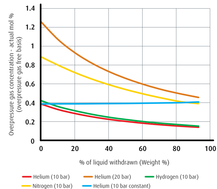
Figure 4: Overpressure gas concentration in liquid phase – actual Mol %
