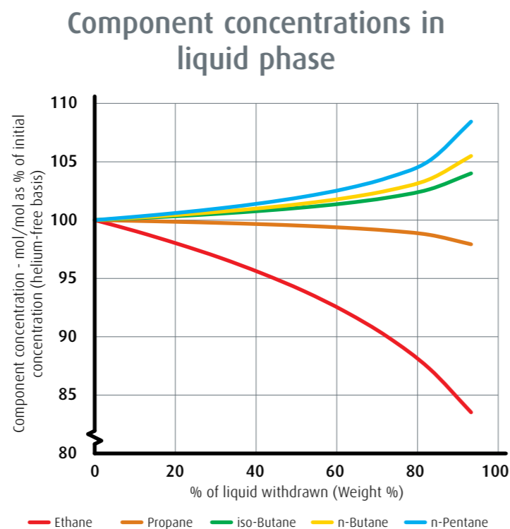
Figure 1: Liquid phase concentrations during cylinder use
