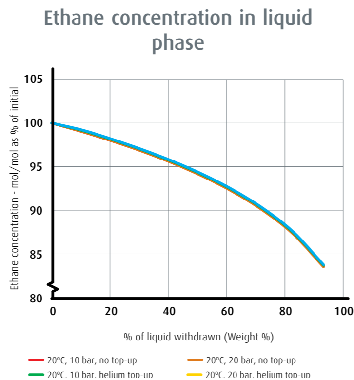
Figure 3: Ethane liquid phase concentrations during cylinder use – top up of pressure
